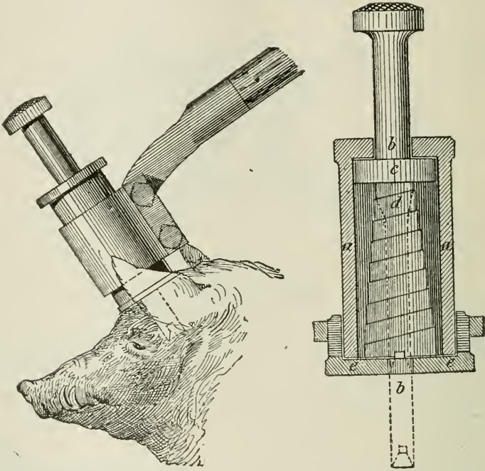
Kleinschmidt's spring bolt apparatus for killing hogs (half natural size).
